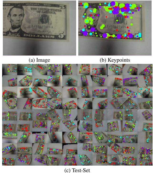
Figure 5. CurrencyDetector process: (a) Scanned image. (b) Detected features. (c) Montage image showing our test set with detected features - different colors represent different classes.
