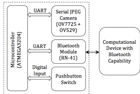
Figure 4. Overview of the EyeRing System.
