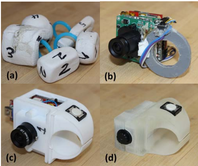
Figure 3. Prototypes of the EyeRing. (a) Clay models used for initial exploration. (b) First working prototype. (c) First prototype with plastic casing. (d) Second prototype.
